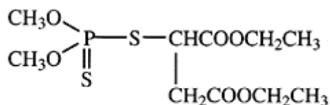
Malathion
