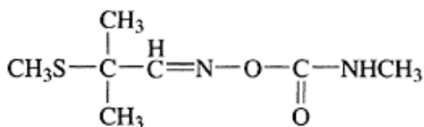
Aldicarb
